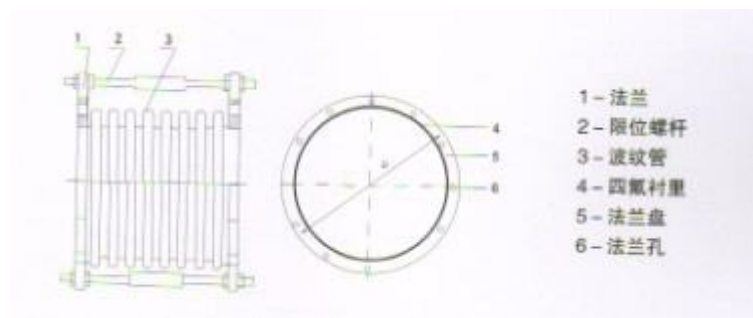
1.Flange 2.Limit screw 3.Bellows 4.PTFE lining 5.Flange 6.Flange holes
