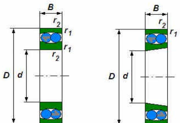
Cylindrical bore
